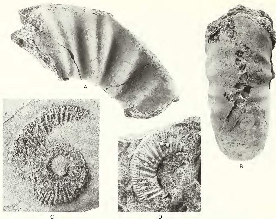
TEXT-FIG. 5. A, B, Dorsoplanitoides ( D. ) bavaricus Zeiss; BMNH C.41284; from bed 91; Chia Gara \times 1 . C, Aulacostephanus cf. volgensis (Vischniakoff); BMNH C.41292; from bed 81; Chia Gara, \times 1 . D, Orthosphinctes desmoides (Wegele); BMNH C.41291; from bed 83; Chia Gara, \times 1.5 .
